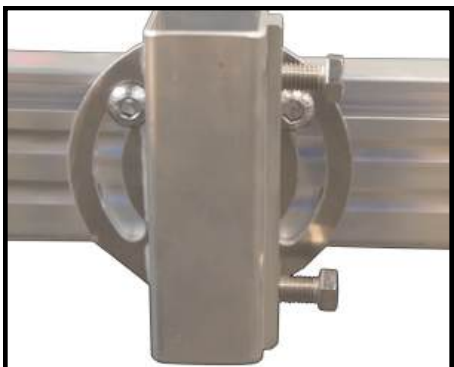
MODULAR DOCK LEG SUPPORT
